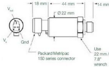
Packard Metripac connector
