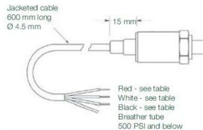
Cable assembly
